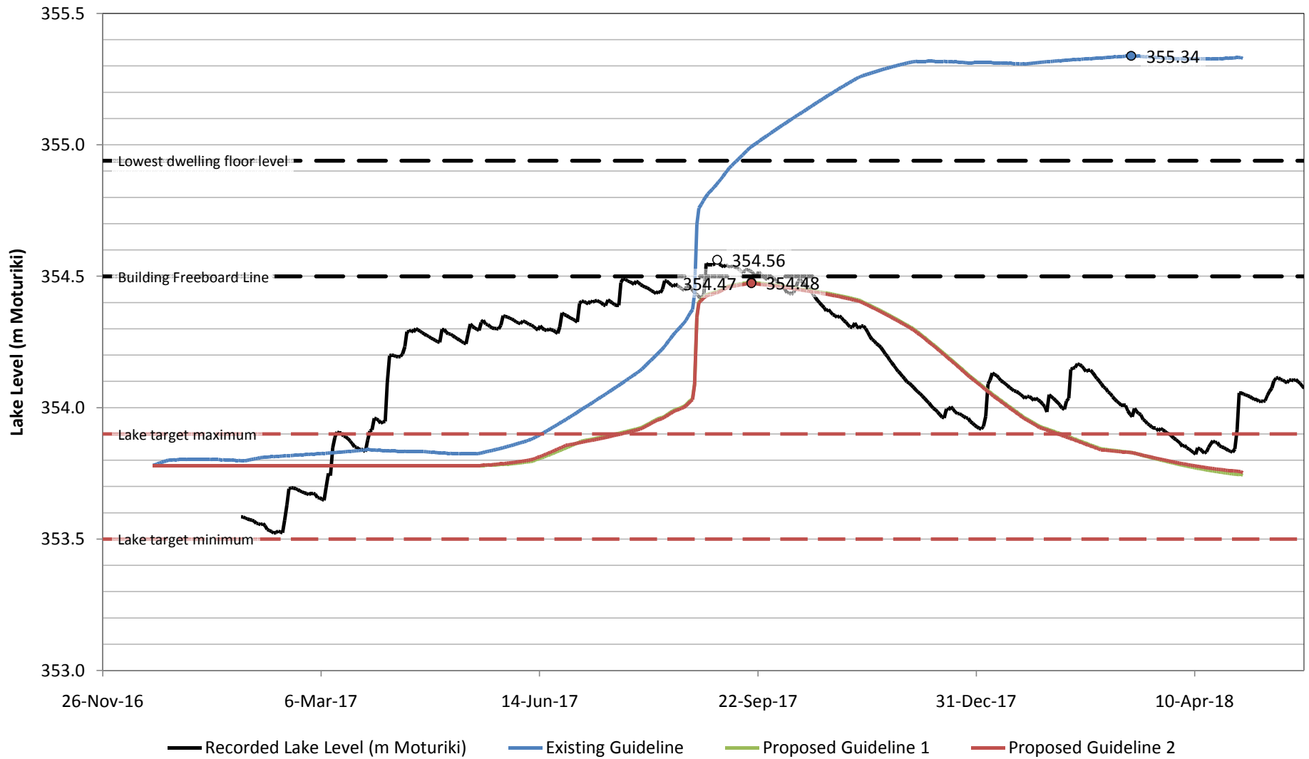
Lake level vs time for 1% AEP design rainfall with "2090 mid-wet" climate scenario
