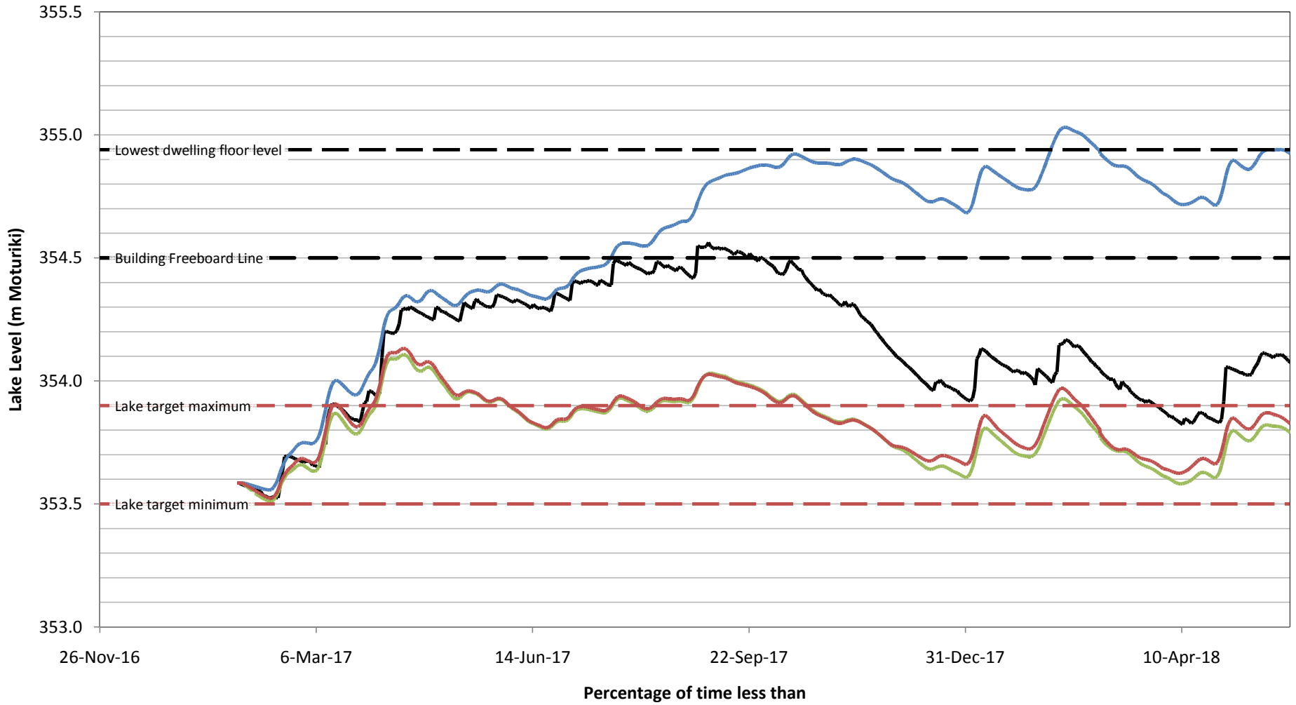
Lake level duration curves for time-history scenarios Feb 2017 to May 2018
