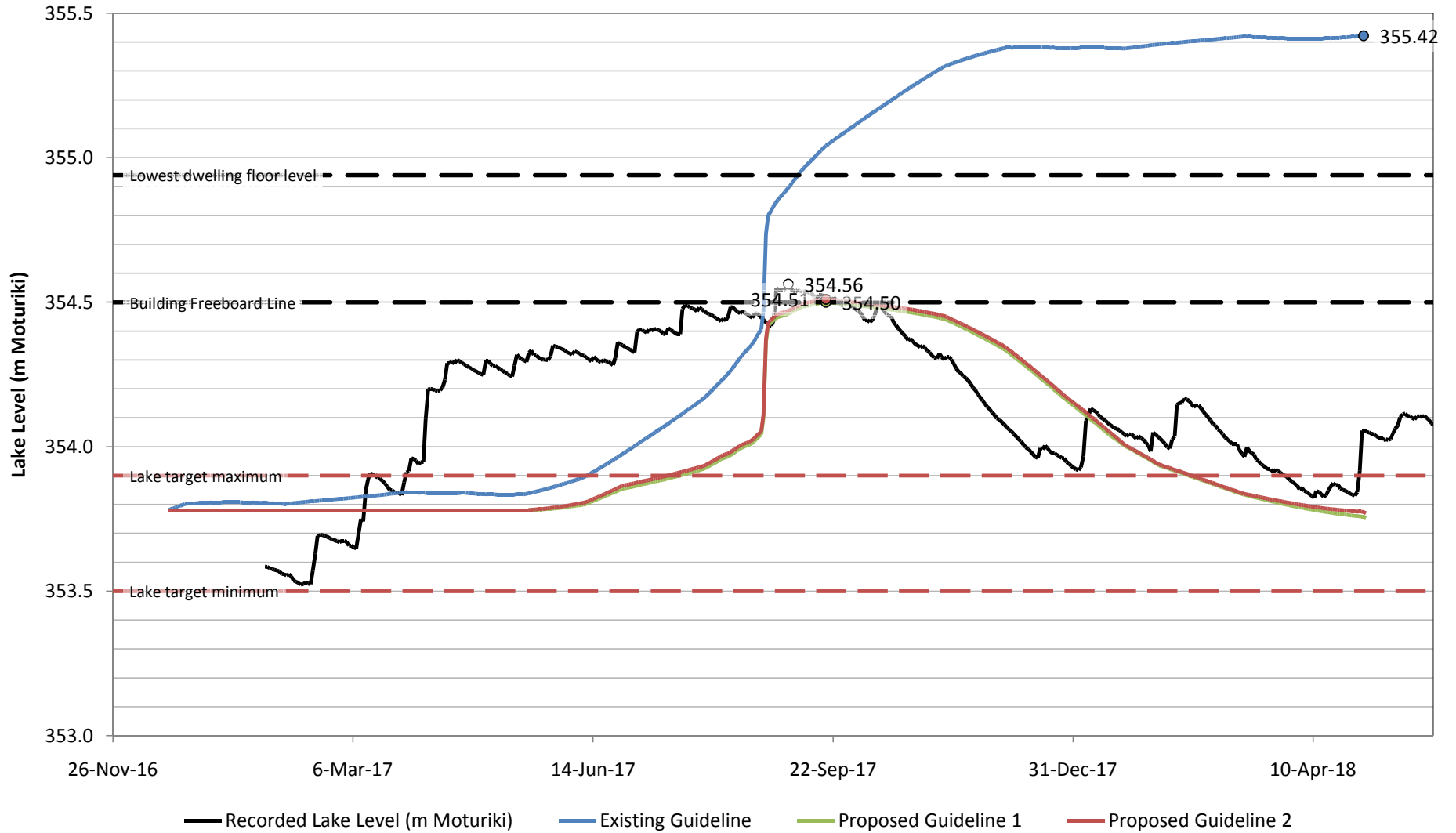
Lake level vs time for 1% AEP design rainfall with "2040 high-wet" climate change scenario
