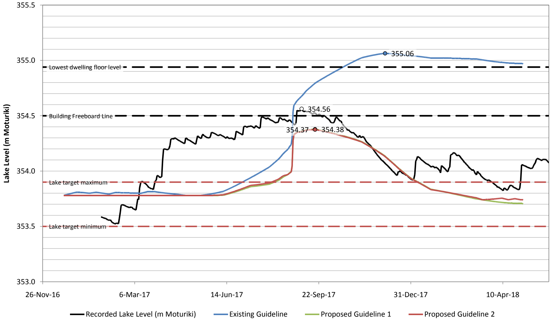
Lake level vs time for 1% AEP design rainfall with "2040 mid-wet" climate change scenario
