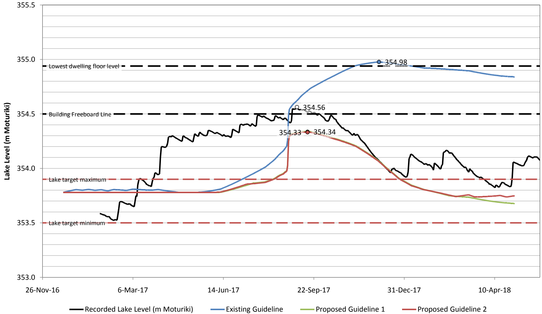
Lake level vs time for 1% AEP design rainfall with present-day climate scenario
