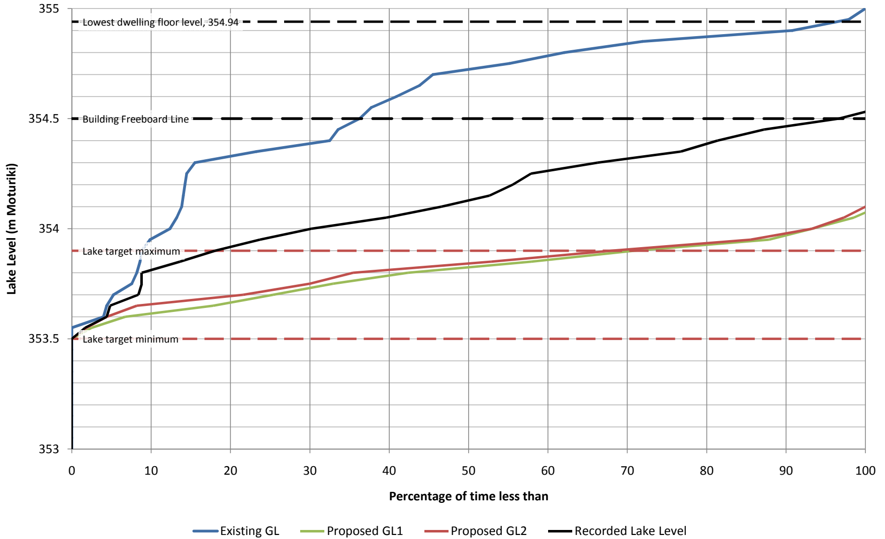
Lake level duration curves for time-history scenarios Feb 2017 to May 2018
