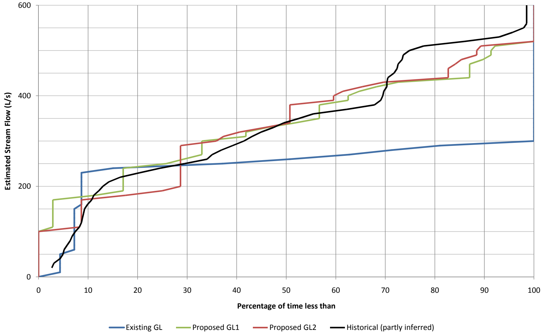
Stream flow duration curves for time-history scenarios Feb 2017 to May 2018
