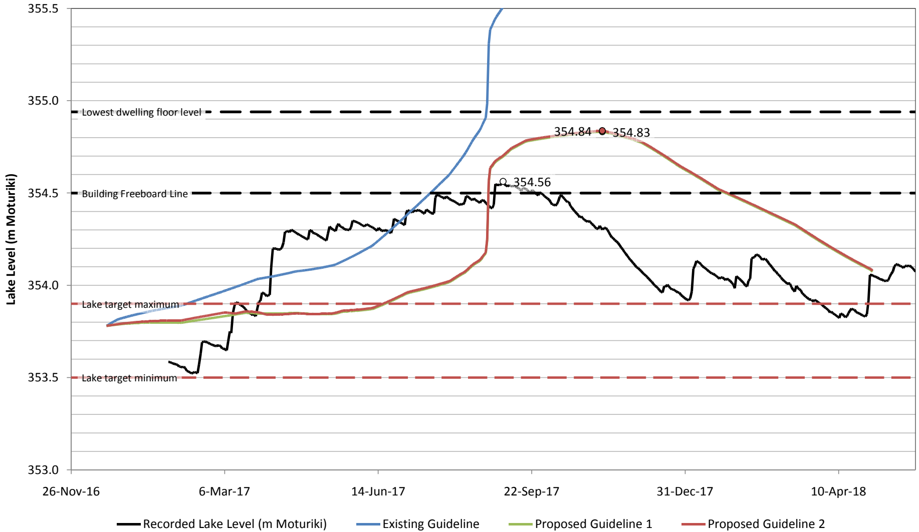
Lake level vs time for 1% AEP design rainfall with "2090 high-wet" climate scenario
