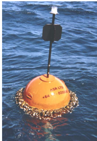
Figure 2.6 Large steel radar-reflecting buoy used to mark the long term ADP deployment sites offshore from Pukehina and Opotiki
