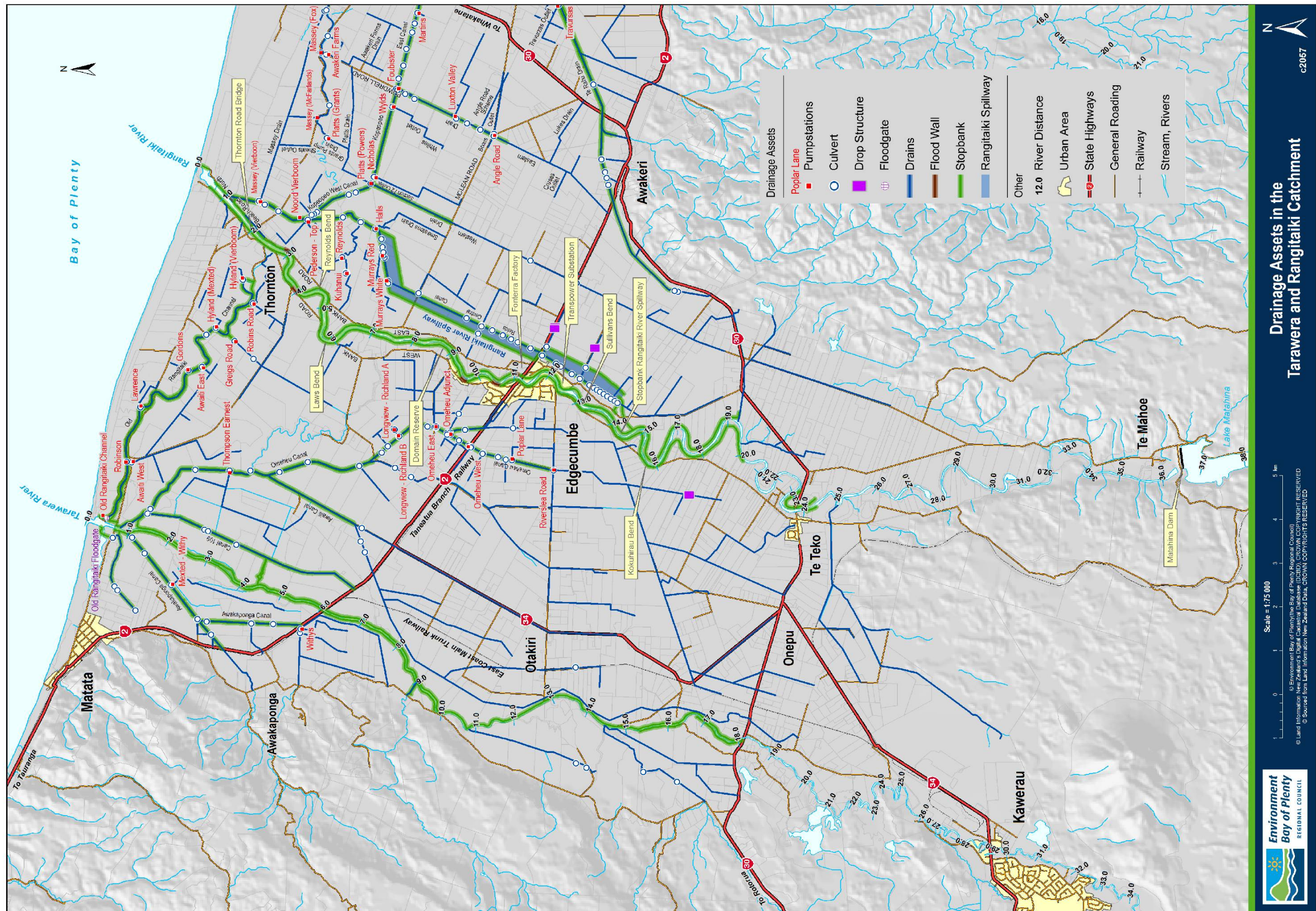
Figure A1.1 Location plan of flood protection assets in Rangitaiki River Scheme.
