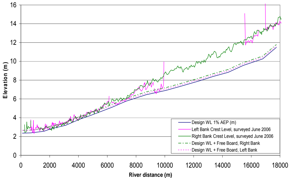
Figure 2.1 Flood levels in Tarawera River below State Highway 30 and stopbank crest levels (from Everitt and Medwin, 2005).
