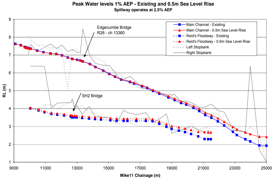
Figure 2.2 Modelled maximum water levels under existing and predicted sea level rise of 0.5 m (from OPUS, 2007). Levels exclude freeboard.
