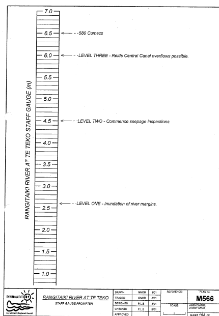
Figure 1.13 Flood warning chart for the Rangitaiki River based on the Te Teko gauge readings.
