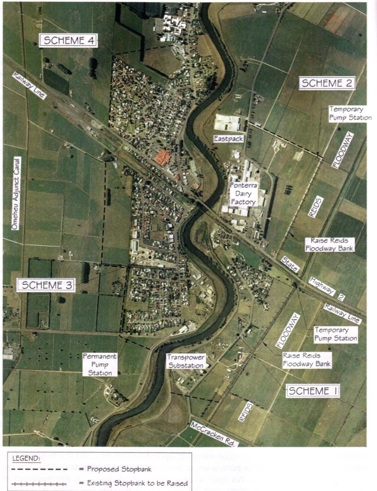
Figure 1.11 Edgumbe flood defence options (OPUS, 2007)
