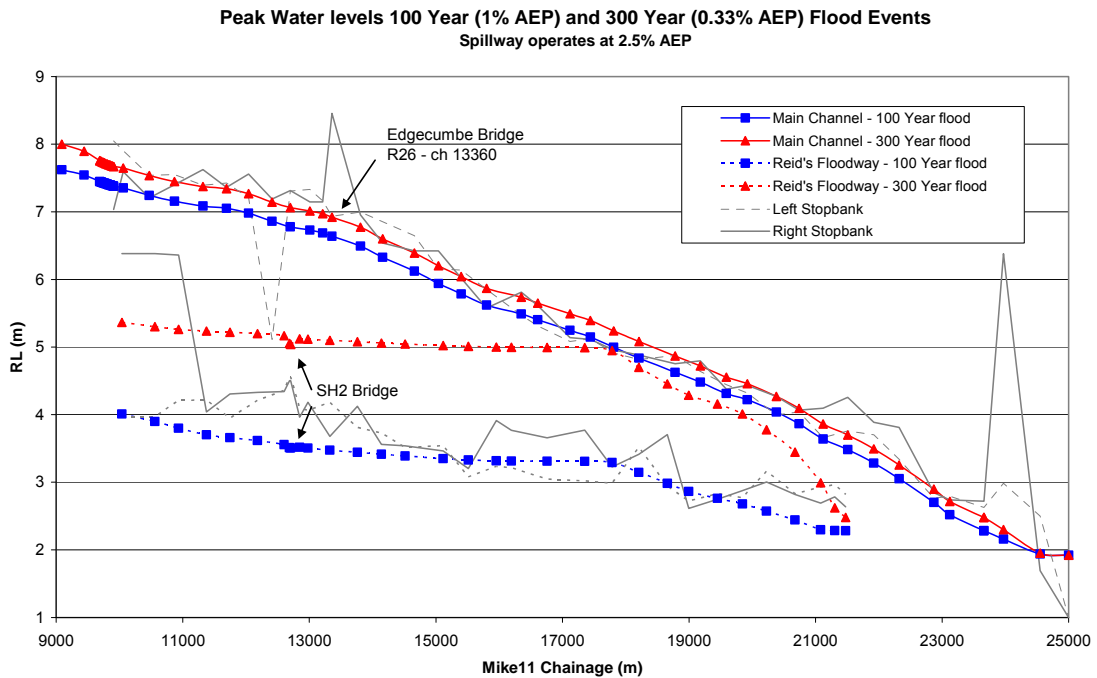
Figure 2.3 Modelled maximum water levels under 100 and 300 year flood events (300 year flood predicted to be future 100 year flood in 2080) (from OPUS, 2006). Levels exclude freeboard.
