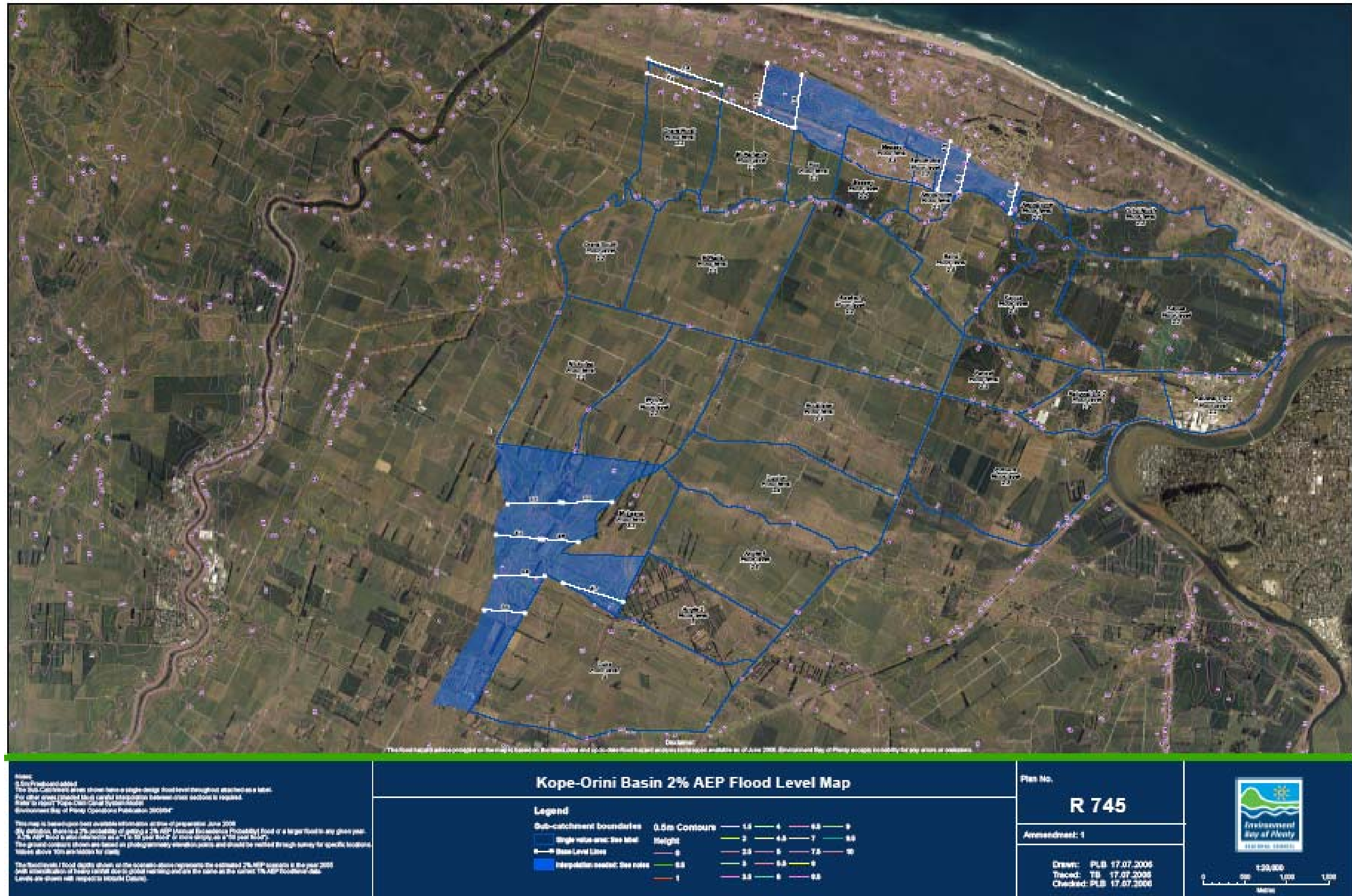
Figure A2.3 Flood depth and extent in Kope Orini Basin during a 50 year flood event (based on 2055 rainfall figures an envelope of maximum flood levels from five scenarios) (Plan R745).
