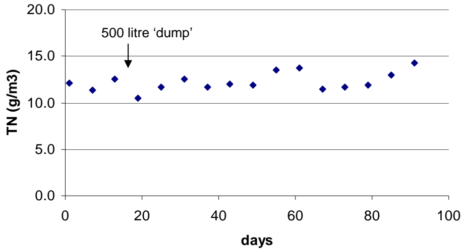
Figure 1 Graph of total nitrogen results over the TN evaluation period
