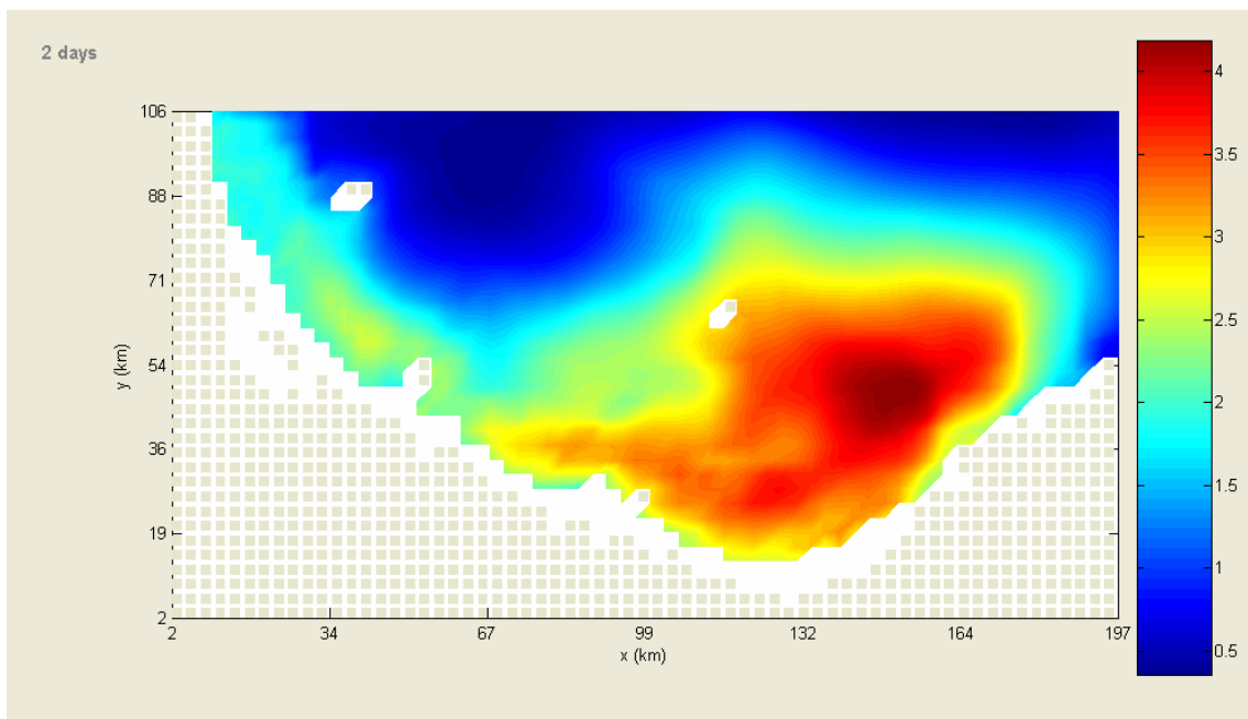
Figure 28. Modelled Seasonal averaged (February-March-April) phytoplankton chlorophyll-a (mg/m 3 ) at 25 m water depth within the Bay of Plenty with No Mussel farm
